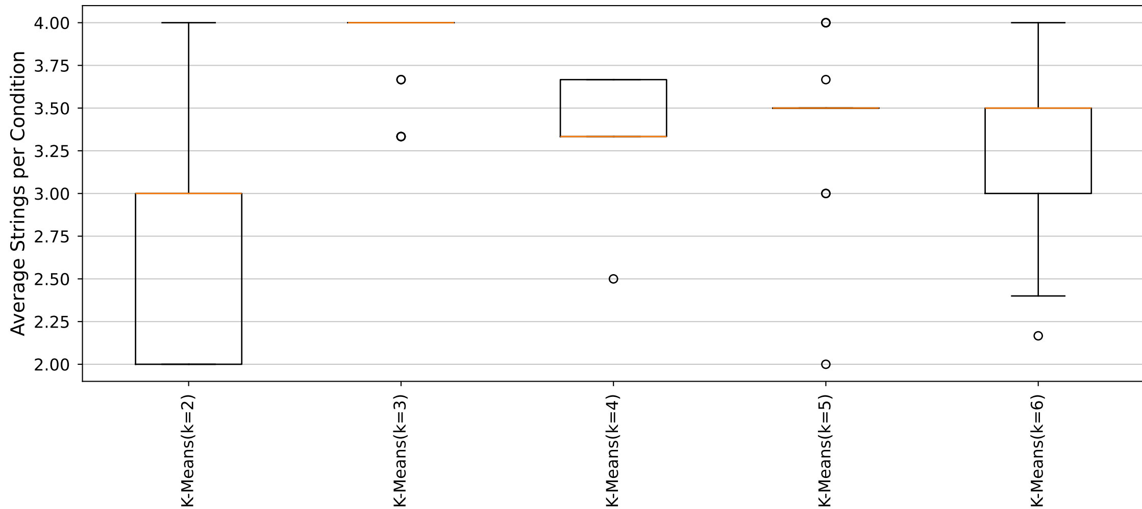
YARA Rules Average Strings per Condition Distribution (Cluster33_Size6 dataset)
